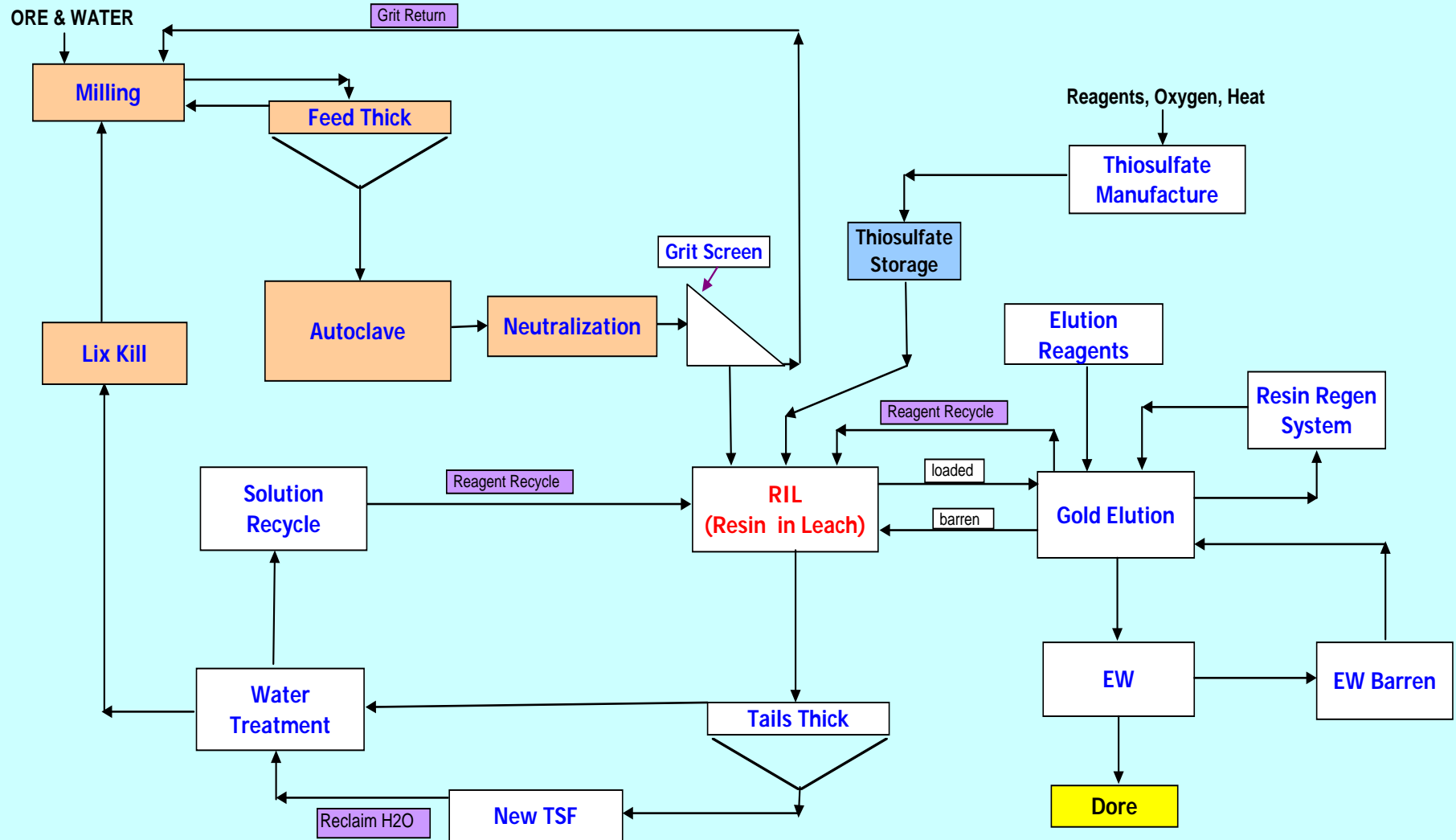
Goldstrike TCM Leach Block Diagram
