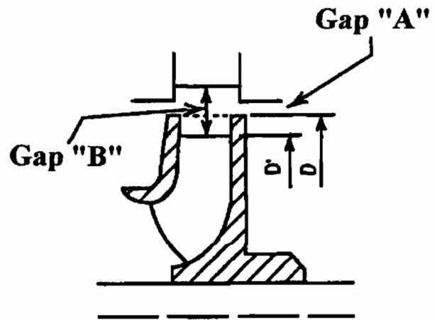
Figure 1. Impeller to Casing Gap "A," Gap "B" Relationship.
