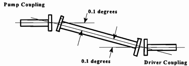
Figure 7. Alignment Tolerance Expressed in Degrees.
