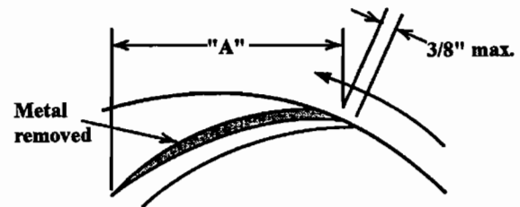
Figure 1. Impeller to Casing Gap "A," Gap "B" Relationship.
