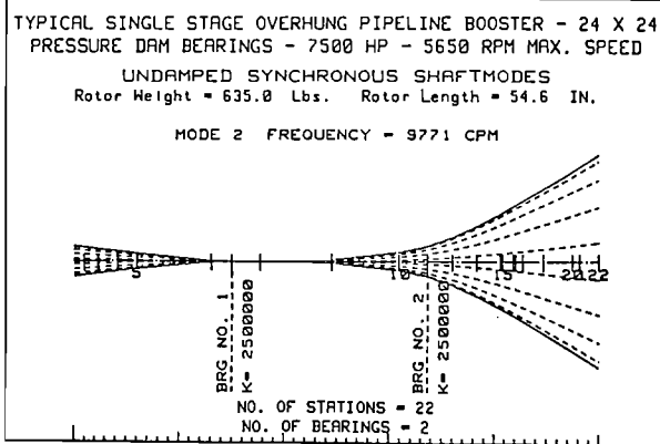
Mode diagrams and rotor model; first and second modes or pivotal
