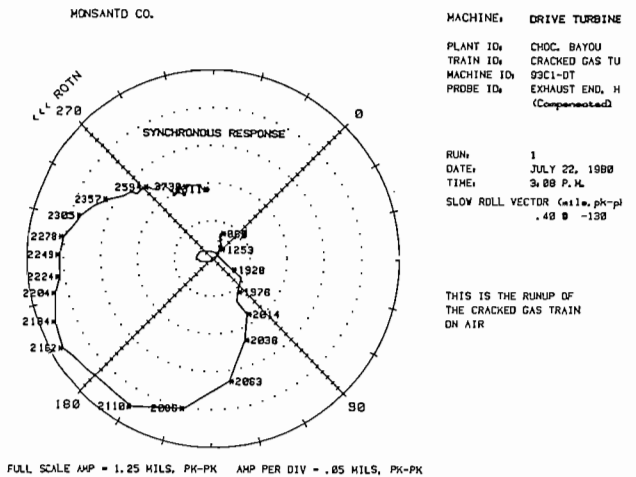
Figure 13. Polar Plots and Bode Plots from Tracking Filter.
