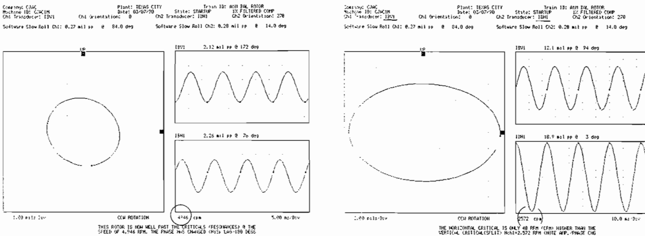
Figure 21. Orbit and Timetraces at 2572 RPM (Horizontal Critical) and 4946 RPM.
