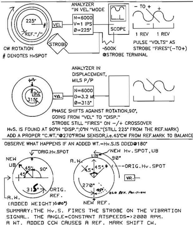
Figure 4. Phase Relationship with Strobe System and Velocity Sensor.
