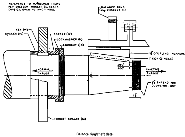
Figure 38. Balance Ring for Overhung Compressor. Similar built, with care, for pumps.
