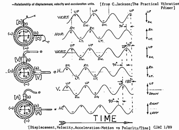
Figure 1. Relationships of Displacement, Velocity, Acceleration, and Sensors.
