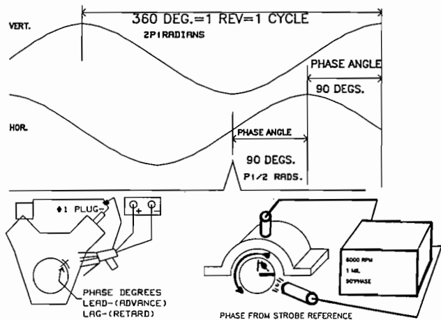
Figure 4. Phase Relationship with Strobe System and Velocity Sensor.
