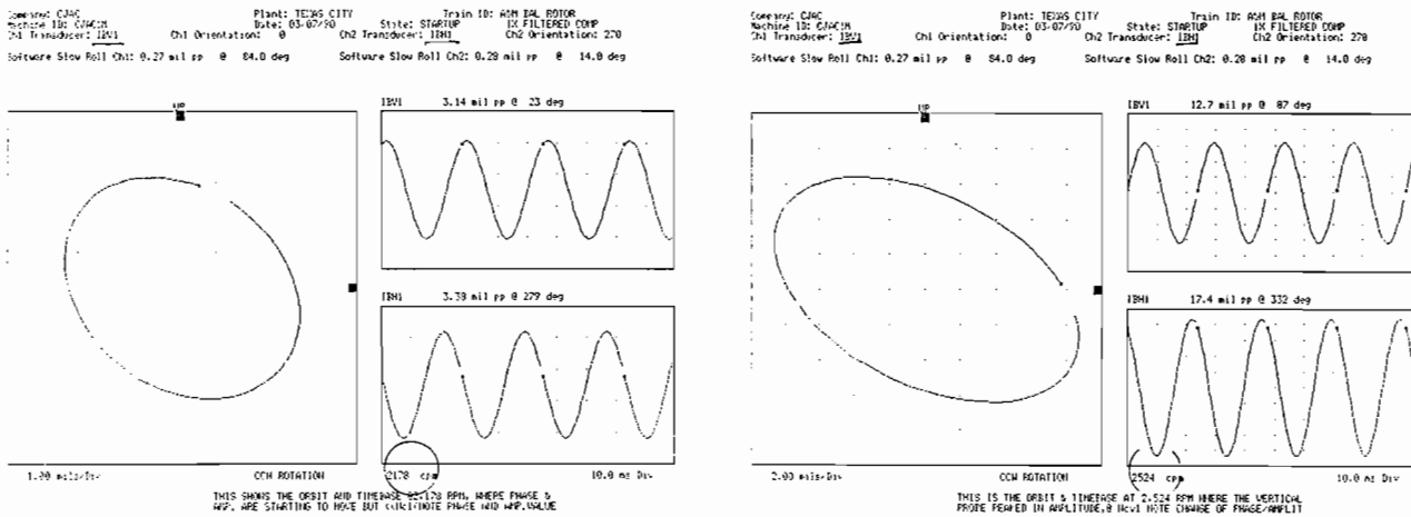
Figure 20. Orbit and Timetraces at 2178 and 2524 RPM (Vertical Critical).
