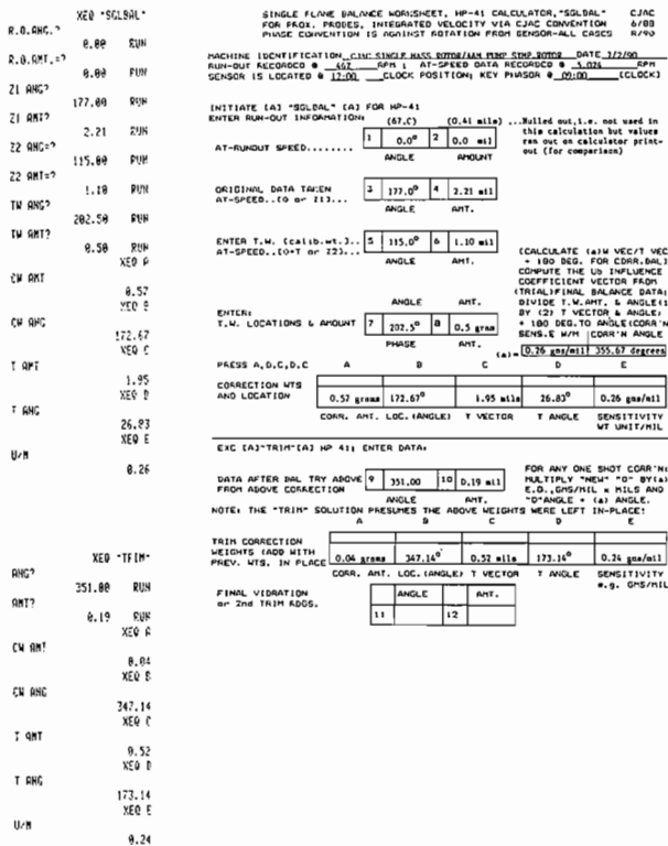
Figure 23. Balance Record Sheet with All Solutions + Calculator Print Out of SGLBAL.
