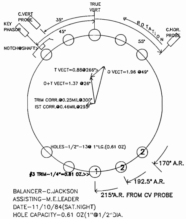
Figure 36. Balance Plane and Vector Layout for Balance In Situ of Overhung Compressor.
