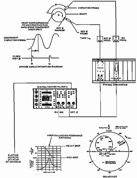
Bode & Polar Outputs from a Tracking Filter (BNC's DVF-2 or 3) [Courtesy Bently Nevada Corp.]
