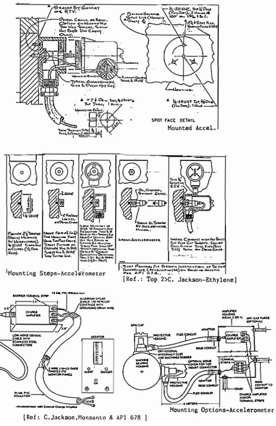
Figure 6. Mounting of Accelerometers—Jackson and API 678.
