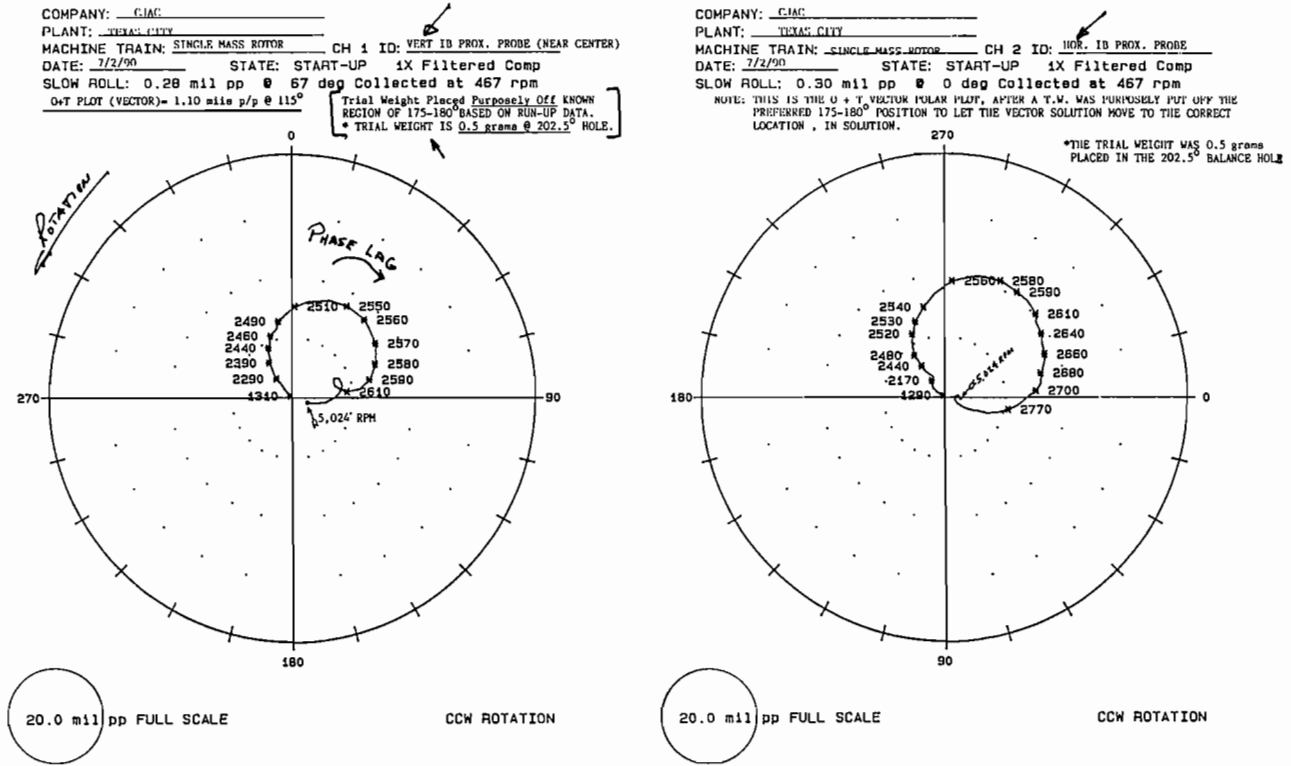
Figure 26. Polar Plots of Vertical/Horizontal Sensors with 0.5 gm at 202.5 degrees (0 + T Vector).
