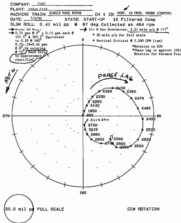
Figure 22. Polar Plots of Vertical (Used to Balance) and Horizontal for 0 Vector to Speed.
