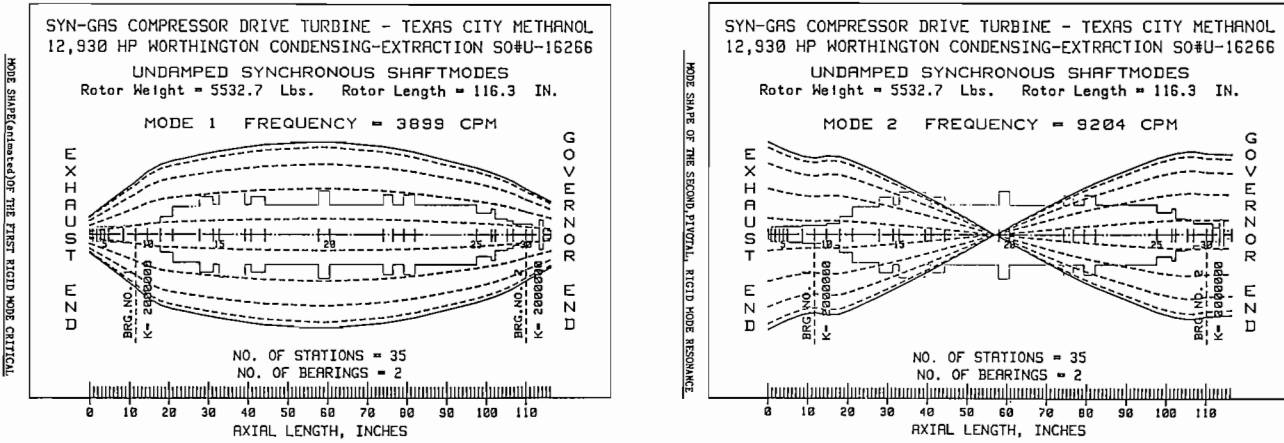
Figure 32. First and Second Mode Shapes, Animated, for Steam Turbine Balance Data. C. Jackson.
