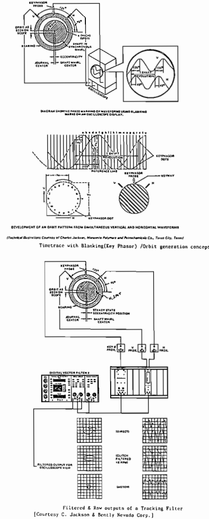
Figure 10. Proximity Signals to Scope and through Tracking Filter.
