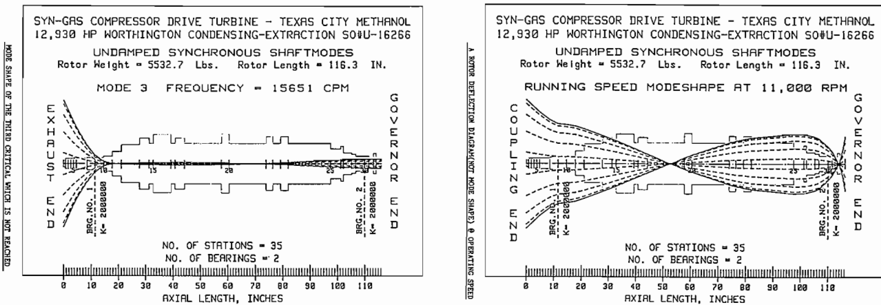
Figure 33. Third Mode Plus Running Speed Deflection Shape. Jackson and Leader.
