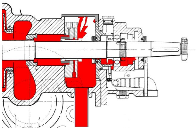
Figure 16 Illustration of High Levels of Process Leakage in Pump Bracket
