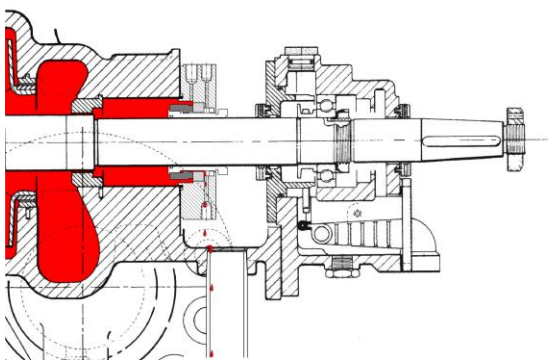
Figure 8 Mechanical Seal Installed in Pump with Drain from Pump Bracket
