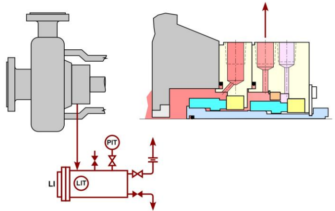
Figure 3 Arrangement 2 with Containment Seal
