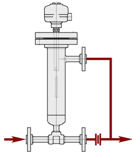
Figure 13 Example of Piping Plan 65 Detection Vessel
