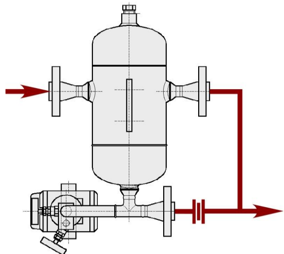
Figure 14 Example of Piping Plan 65 Detection Vessel
