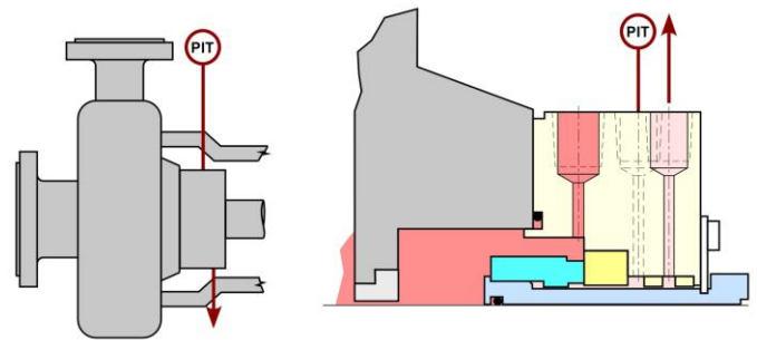
Figure 17 Piping Plan 66A
