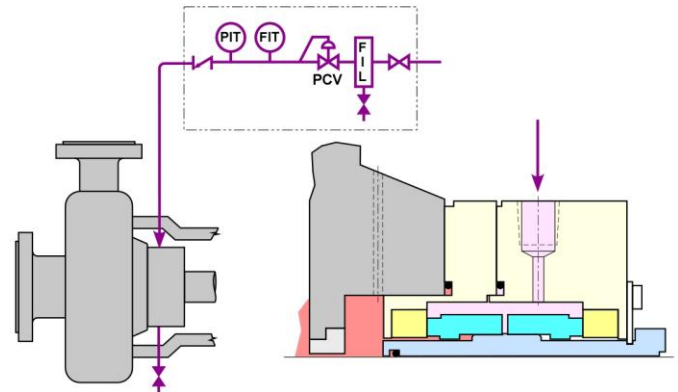
Figure 5 Arrangement 3 with Gas Barrier Fluid
