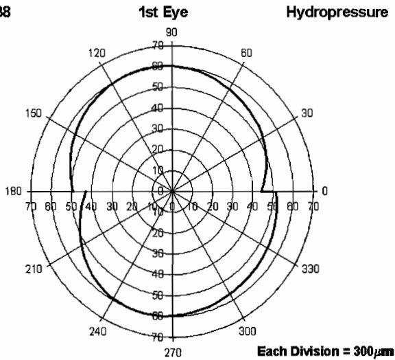
Figure 33. Polar Plot, First Eye—Hydropressure.
