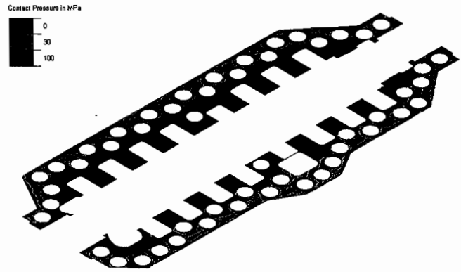
Figure 18. Gasket Compression—Hydropressure.
