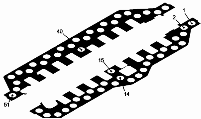
Figure 12. Bolt Location—Definition.
