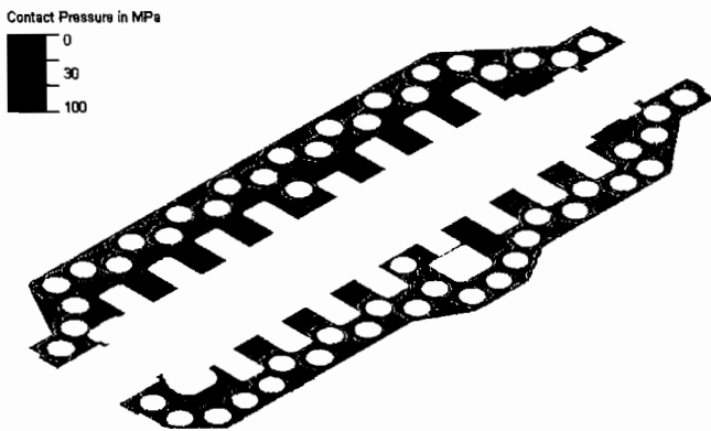
Figure 17. Gasket Compression—Bolt Pretension.
