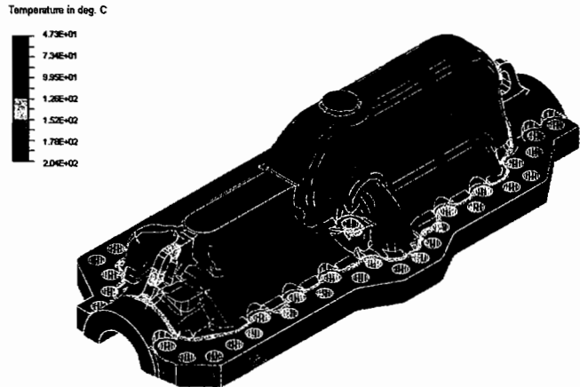
Figure 7. Upward Transient, Temperature Field after t = 16 \text{ min } 30 \text{ sec} .
