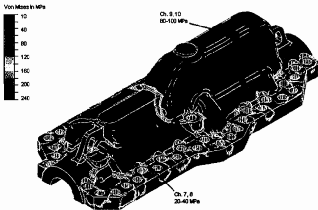
Figure 23. Top Half Von Mises Stress During Operating Pressure.
