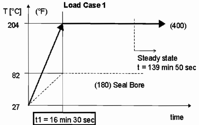
Figure 6. Applied Temperatures to Wet Areas.
