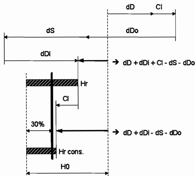
Figure 35. Clearance Vector Diagram.
