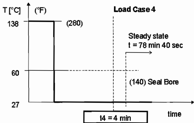
Figure 11. Applied Temperatures to Wet Areas.
