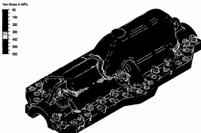
Figure 13. Von Mises Stress on Top Half During Hydrotest Pressure.
