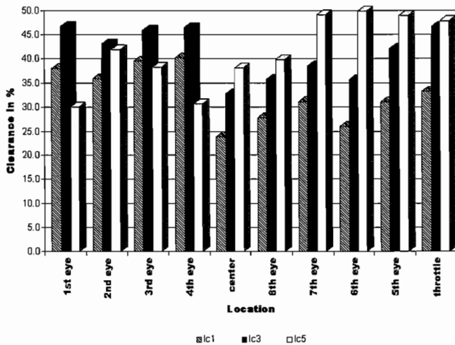
Figure 37. Remaining Clearances at Annular Seal Locations, Case Ring Bound.
