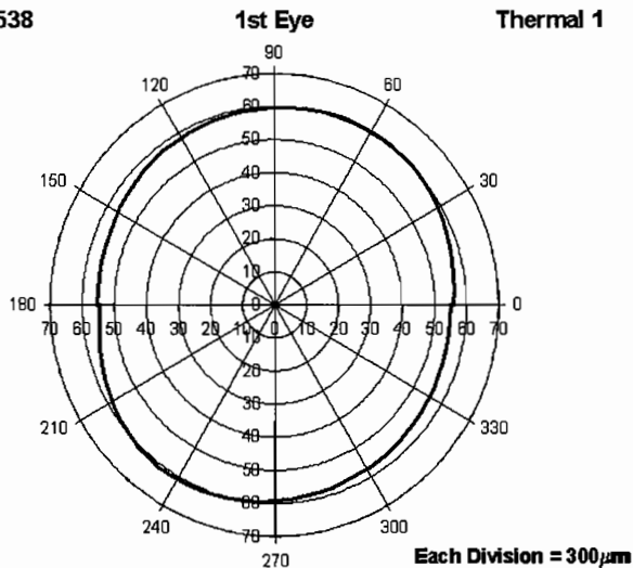
Figure 34. Polar Plot, First Eye—Thermal Load Case 1.
