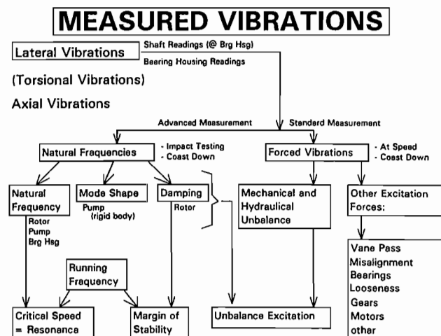
Figure 1. Resonant and Stability Problems Vs Forced Vibration Problems.
