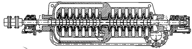
Figure 3. Cross Section of Pump B.
