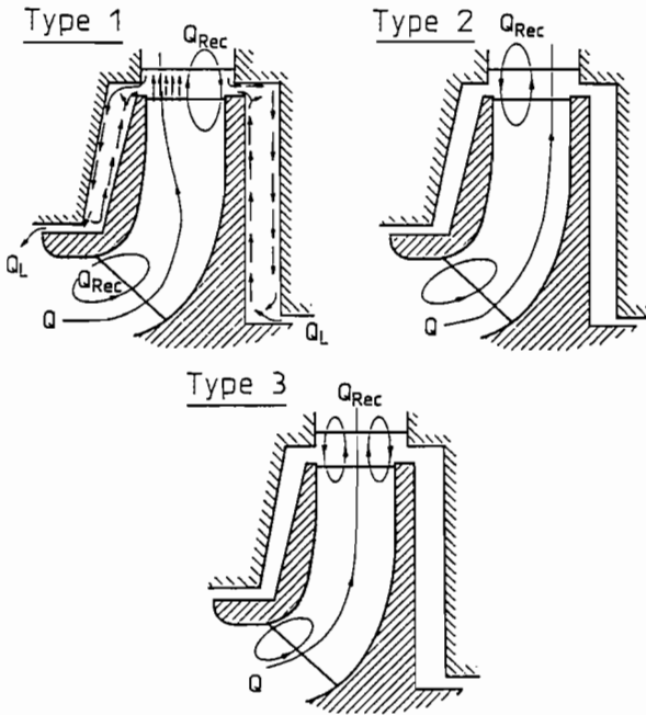
Figure 9. Part Load Flow Patterns.
