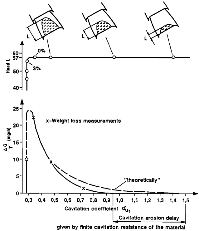
Figure 14. Cavitation Bubbles Vs NPSH.
