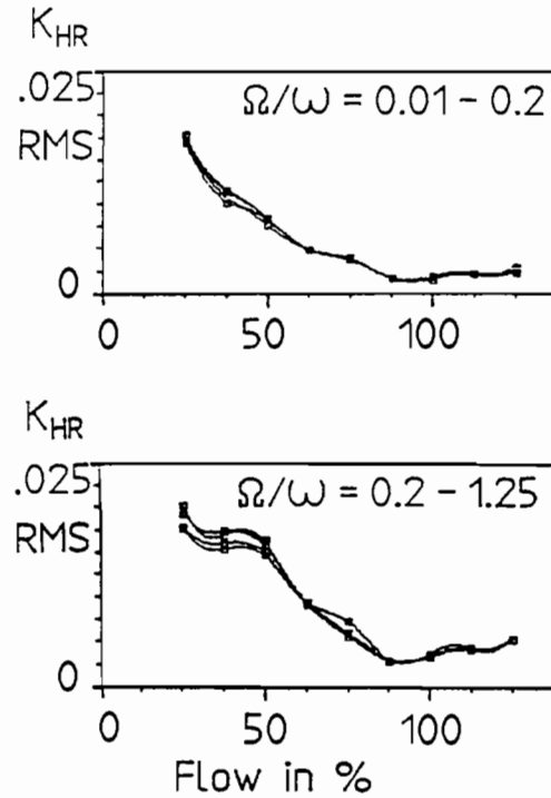
Figure 12. RMS-Values in Two Frequency Bands of Normalized Radial Broad Band Forces.
