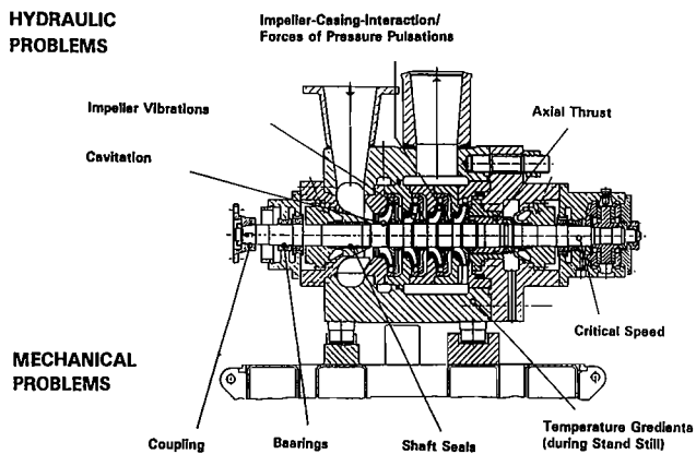
Figure 2. Different Origins of Loading Forces (Cross Section of Pump A).
