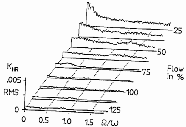
Figure 11. Spectra of Normalized Radial Broad Band Forces, for Various Flows.
