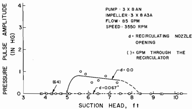
Figure 12a. Small Process Pump Surge at 85 GPM, Pressure Pulse Amplitude.
