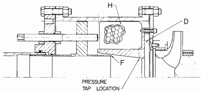
Figure 5. Backflow Recirculator for 3 × 8 AN, Small Process Pump.
