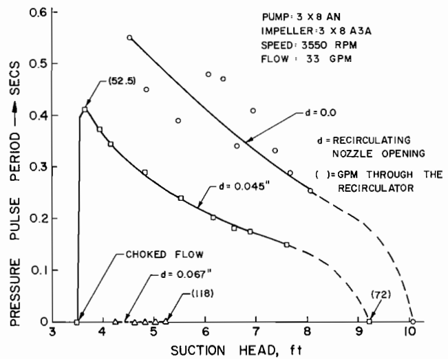
Figure 10b. Small Process Pump Surge at 33 GPM, Pressure Pulse Period.
