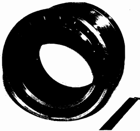
Figure 15. View of Backflow Recirculator Insert as Seen from the Impeller Eye or Downstream End.
