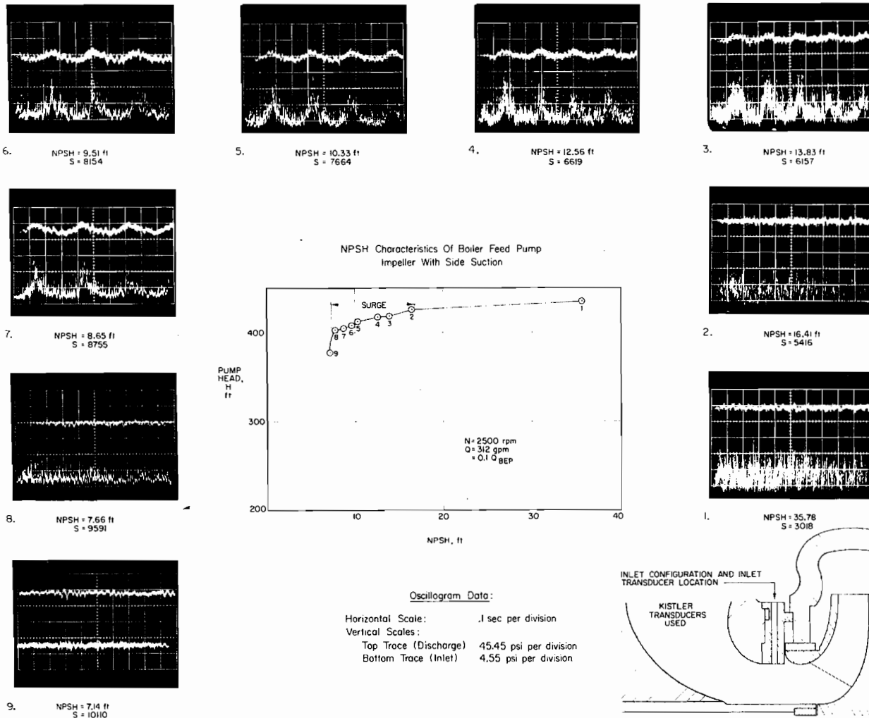
Figure 20. Pressure Pulsation Amplitude-Versus-Time Oscilloscope Traces for Multistage Pump Impeller and Inlet. Each Photograph Corresponds to a Numbered Point on the Head-Versus-NPSH Curve. The Flow Rate Is 10 Percent of That at the Best Efficiency Point.
