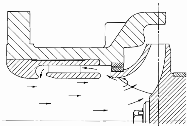
Figure 14. Sectional View of Ingersoll-Rand Process Pump, Model 6 x 10 x 12 ALB, with Backflow Recirculator Insert.
