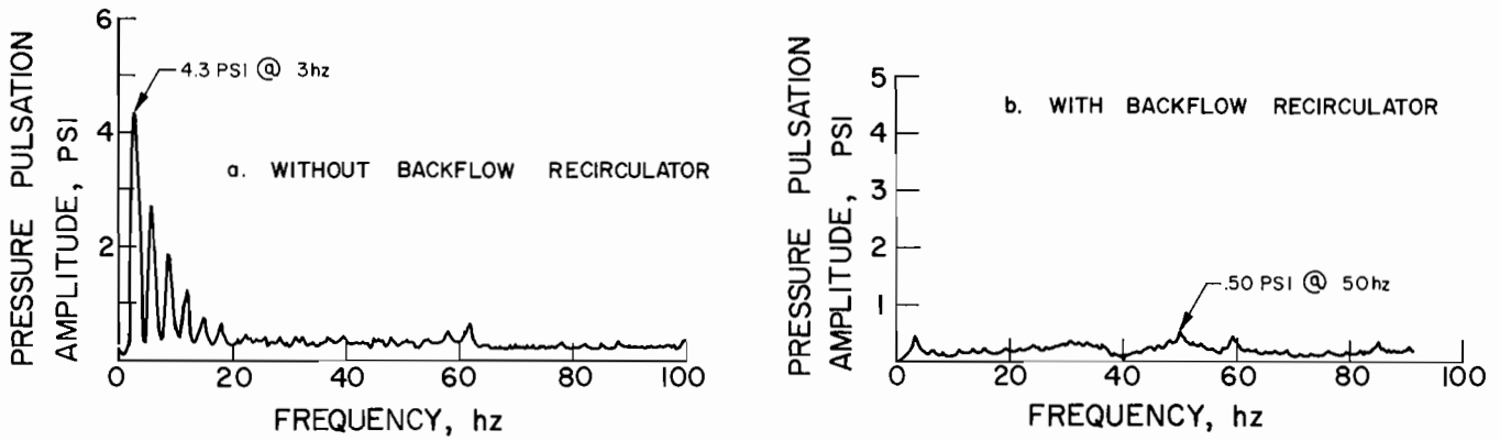
Figure 19 a,b. Inlet Pressure Pulsation Amplitude-Versus-Frequency at 400 GPM (16 Percent of BEP Flow Rate) and 18 Feet NPSH (Near the Head Breakdown Condition).
