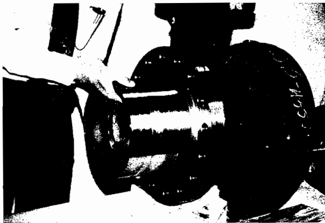
Figure 16. Photograph of the 6 x 10 x 12 ALB Centrifugal Pump Showing the Backflow Recirculator Partially Inserted into the Suction Nozzle.
