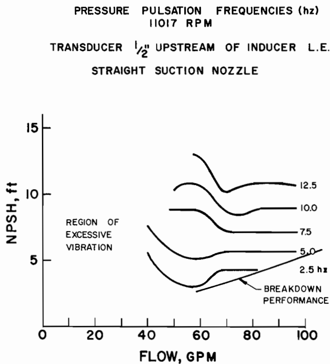
Figure 25. Inlet Pressure Pulsation Frequencies for Test Pump.
