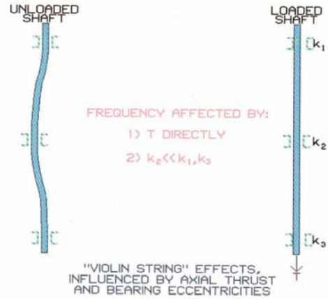
Figure 16. Vertical Pump Lineshaft Rotor Behavior
