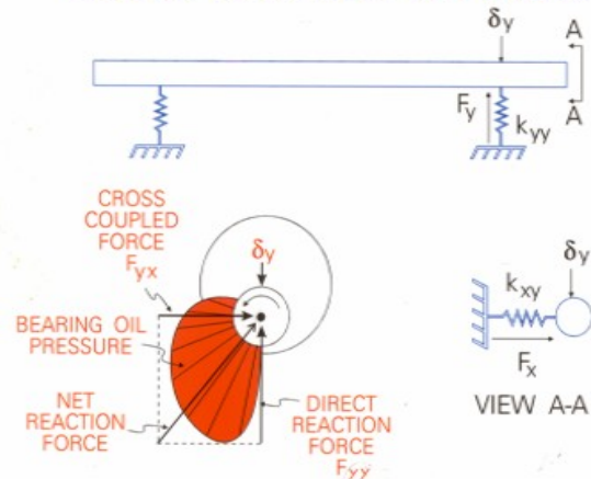
Figure 10. Cross-Coupled Stiffness
