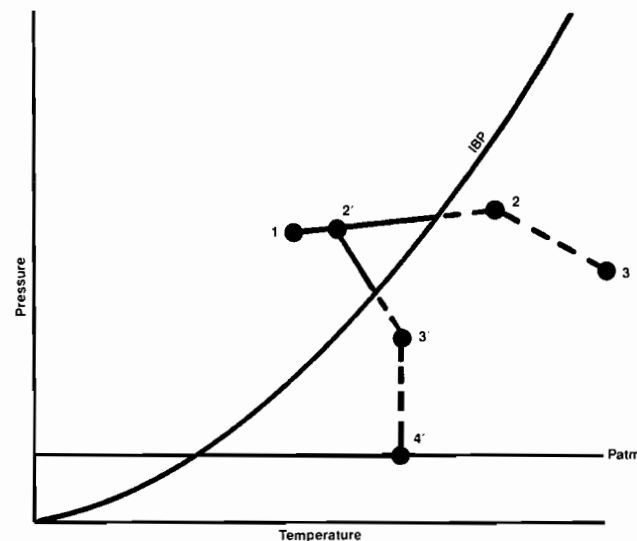
Figure 4. Sealed Fluid Above its Atmospheric Boiling Point. 1) Pumped Fluid, 2) Stuffingbox, wide face seal, vaporization and failure, 3) Seal Face, wide face seal, high temperature, 2') Stuffingbox, narrow face seal, 3') Seal Face, narrow face seal, 4') Seal Exit, narrow face seal.
