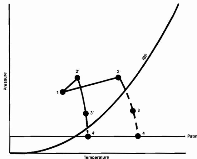
Figure 3. Seal with Vaporization Potential. 1) Pumped Fluid, 2) Stuffingbox, wide face seal, 3) Seal Face, wide face seal, 4) Seal Exit, wide face seal. 2') Stuffingbox, narrow face seal, 3') Seal Face, narrow face seal, 4') Seal Exit, narrow face seal.
