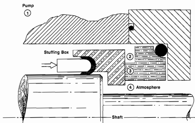
Figure 1. Thermodynamic Reference Points. 1) Pumped Fluid, 2) Stuffingbox, 3) Seal Face, 4) Seal Exit (usually atmospheric).
