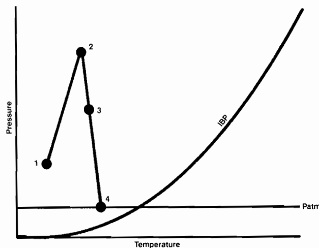
Figure 2. All Liquid Seal. 1) Pumped Fluid, 2) Stuffingbox, 3) Seal Face, 4) Seal Exit.
