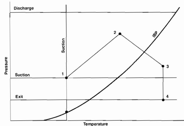
Figure 6. Seal Thermodynamic Plot. 1) Pumped Fluid, 2) Stuffingbox, 3) Seal Face, 4) Seal Exit.
