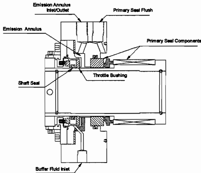
Figure 4. Single Unit Gland.
