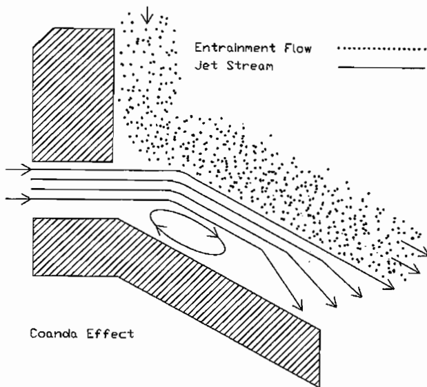
Figure 1. Coanda Effect.
