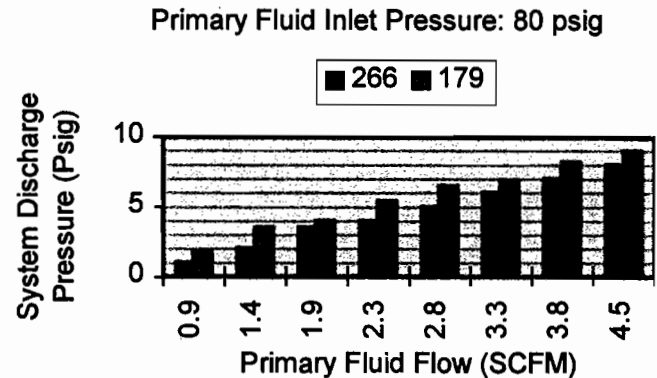
Figure 8. Jet Manifold Sizing Chart.
