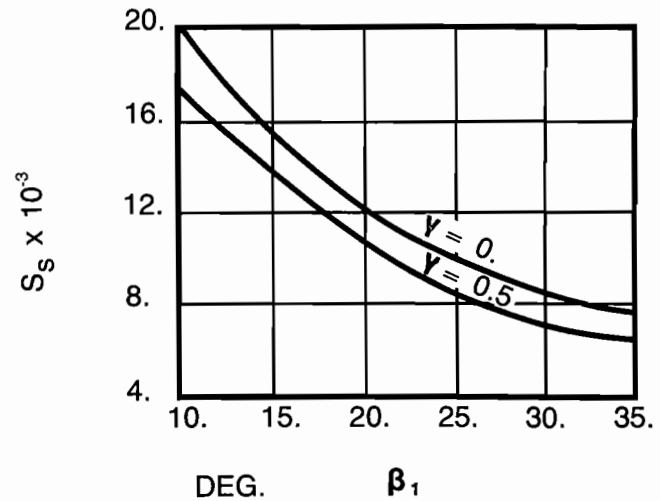
Figure 5. Variation of Suction Specific Speed with Vane Inlet Angle.
