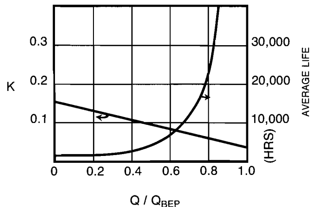
Figure 3. Reduction in Anticipated Average Bearing Life Due to Increasing Radial Loads at Low Flows.
