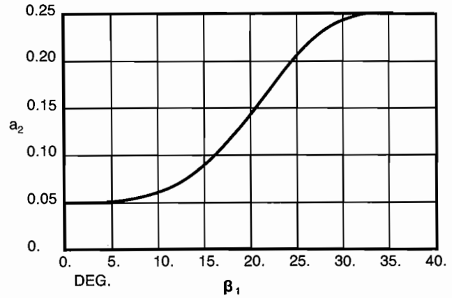
Figure 4. Variation of NPSH Coefficient a_2 with Vane Inlet Angle.
