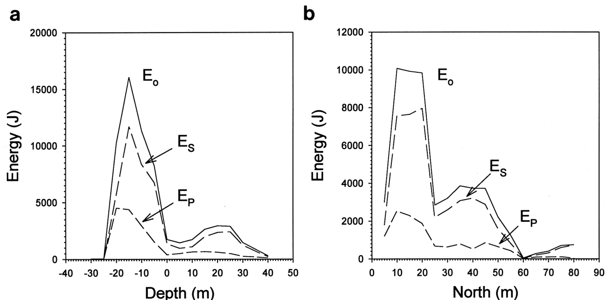
Figure 3: Average total seismic energy ( E_0 ), P-wave energy ( E_P ), and S-wave energy ( E_S ) values based on a 5 m moving window as a function of (a) depth above the excavation base and (b) ahead of the advancing excavation front (north).
