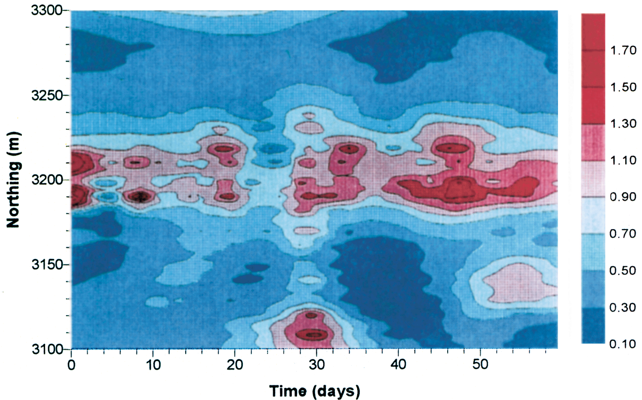
Figure 7: Space-time distribution in northing of the b-values as calculated on a 5 m, 12-hour grid.
