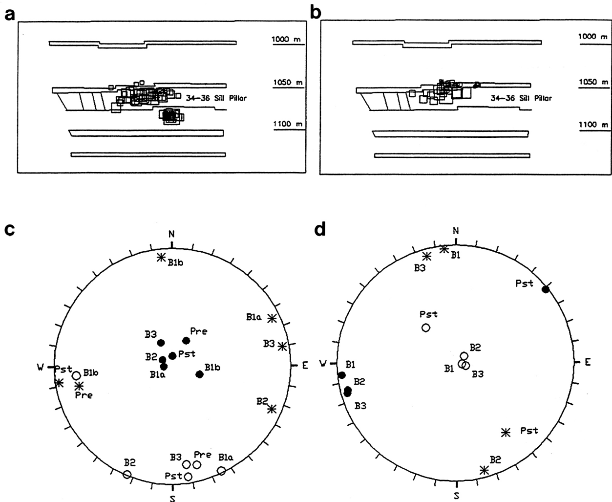
Figure 4: Longitudinal view (looking north) showing the distribution of (a) reverse and (b) normal faulting events for the first blast interval. Principal stress axes ( F_1 — open circles, F_2 — stars, F_3 — filled circles) of the reverse (c) and normal (d) faulting events for the different extraction stages: pre-mining (Pre), blast 1 (B1a for events within the sill and B1b for those below), blast 2 (B2), blast 3 (B3), and post-mining (Pst).
