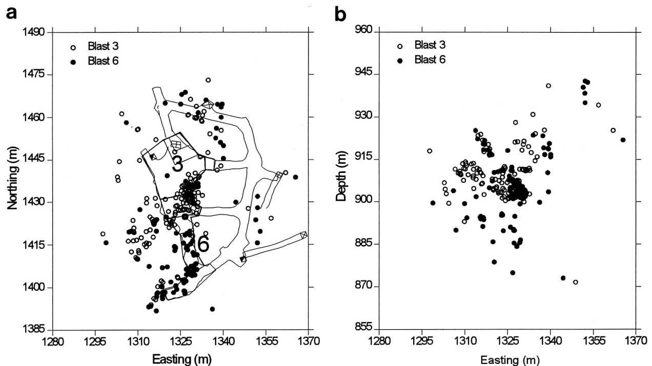
Figure 5: Distribution of seismicity in plan view at (a) mid-sill height and (b) in cross-section for excavation stages 3 (open circles) and 6 (solid circles).
