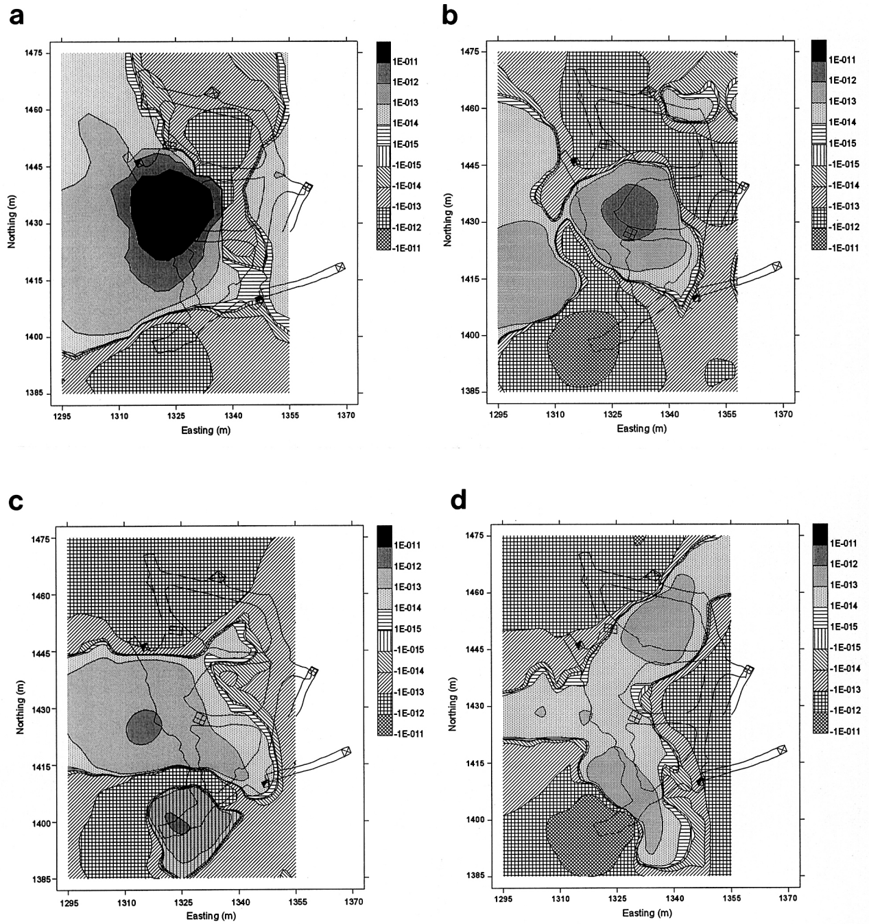
Figure 6: Vertical deformation rate in \text{day}^{-1} for excavation stage 3 at (a) mid-sill height and (b) below the sill, and for excavation stage 6 at (c) mid-sill height and (d) below the sill.
