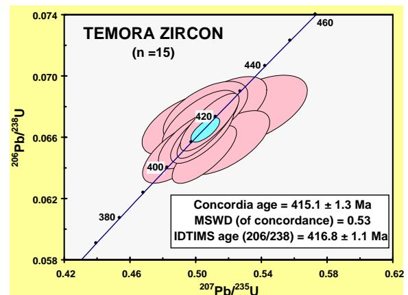
Figure 1: LAM-ICPMS dating of zircons from the Temora granodiorite, illustrating typical precision and accuracy (after Jackson et al., 2004)
