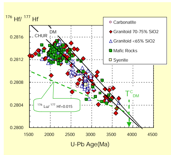
Figure 3: Plot of Hf-isotope composition vs age for detrital zircons from the Carajas area, Brazil. Grains are classified by modelled rock type. Dashed line shows evolution of ^{176}\text{Hf}/^{177}\text{Hf} in 3.9 Ga “average continental crust”. The two mantle evolution lines for ^{176}\text{Hf}/^{177}\text{Hf} are CHUR (CHondritic Uniform Reservoir), representing the primordial undifferentiated mantle values and DM (Depleted Mantle) representing mantle evolution through melt removal (and hence depletion).
