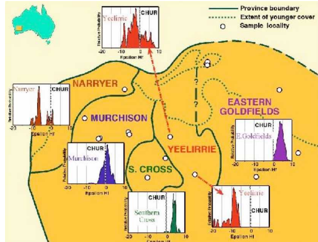
Figure 8: Relative probability histograms of \epsilon\text{Hf} data for zircons with ages of 2.6-2.8 Ga provinces in the Yilgarn Craton, (W. Australia). Note the juvenile character ( \epsilon\text{Hf} > 0 ) of the magmatism in the Eastern Goldfields and Southern Cross provinces, and the major contribution of ancient crust ( \epsilon\text{Hf} < 0 ) in Yeelirrie and Narryer. (Griffin et al., 2004).
