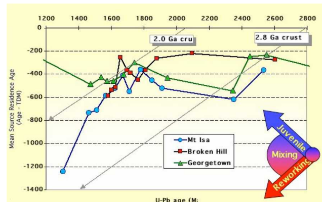
Figure 6: Event Signature diagrams for Mt Isa (Qld), Georgetown (Qld), and Broken Hill (NSW).
