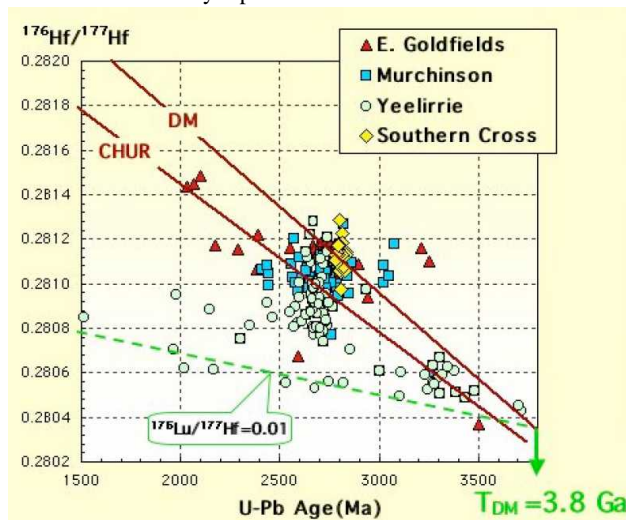
Figure 7: Age-Hf data for detrital zircons from the northern part of the Yilgarn craton, W. Australia
