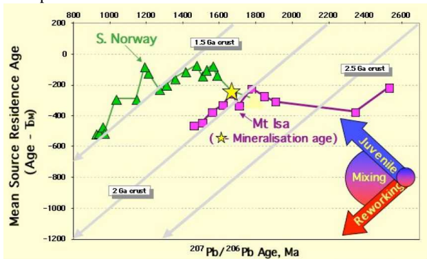
Figure 5: Event Signatures for the Mt Isa Eastern Succession (Queensland, Australia) and S. Norway.
