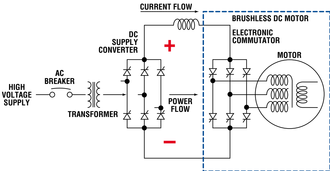
Figure 55 Load commutated variable frequency drive (6-pulse).
