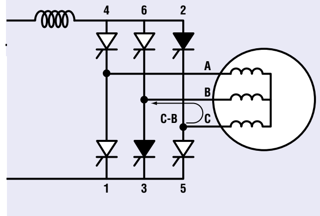
Figure 57 Load Current Path (C-B)
