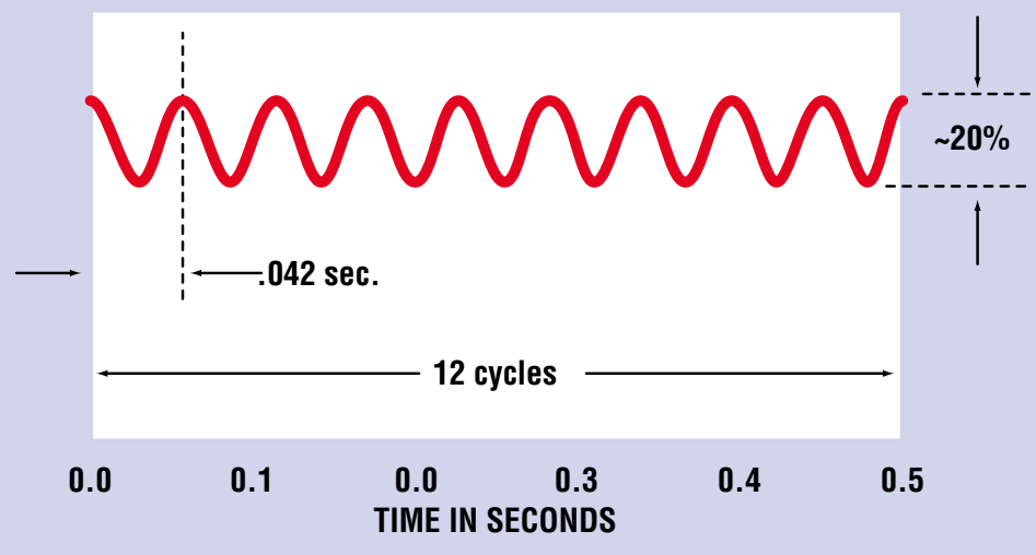
Figure 32 Pulsations in total torque due to reluctance variations in magnetic circuit at 80% speed; 24 Hz. or .042 sec./cycle.
