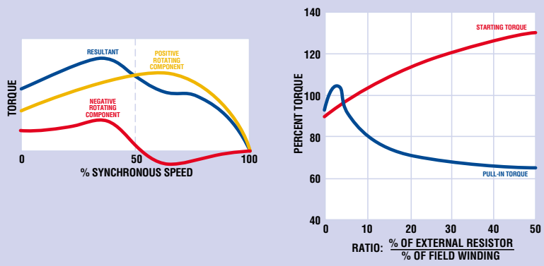
Figure 18 Torque components and resultant torque derived from the field winding of a synchronous motor during starting.
