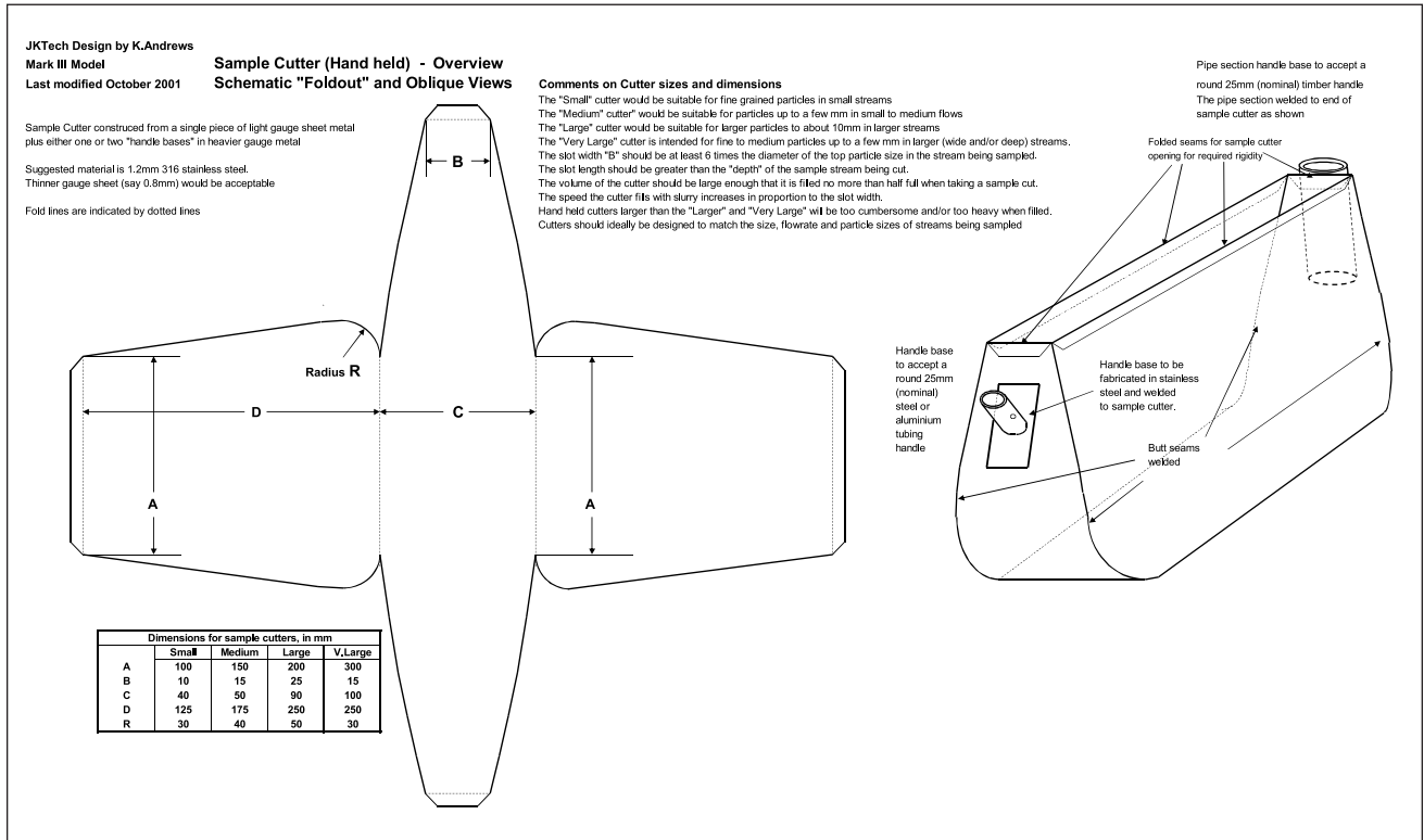
Figure 1. Example Sample Cutter Design (reprinted with permission from JKTech)
